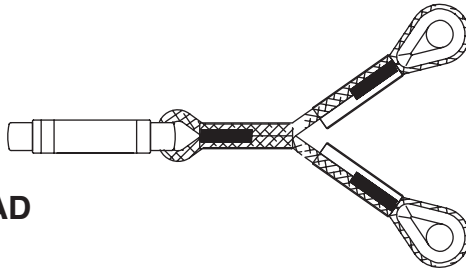
LDA
